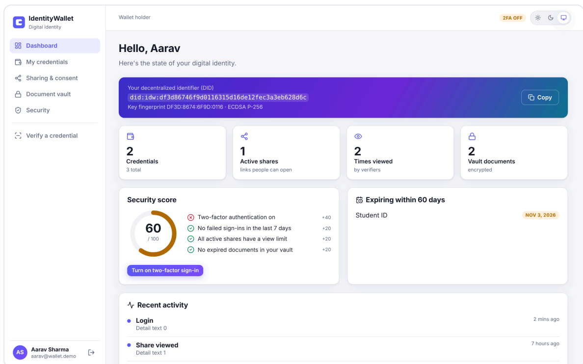
Figure 8.2 — Holder dashboard: DID, statistics, security score, activity
